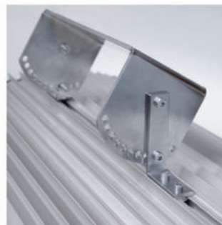
Fix ceiling mounting
