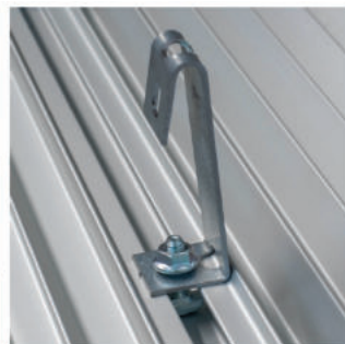
Steel wire mounting
